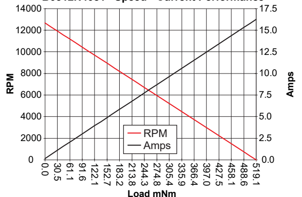
B0512N4081 Speed - Current Performance
