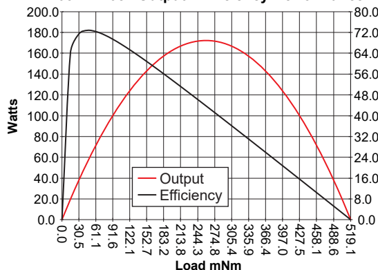
B0512N4081 Output - Efficiency Performance
